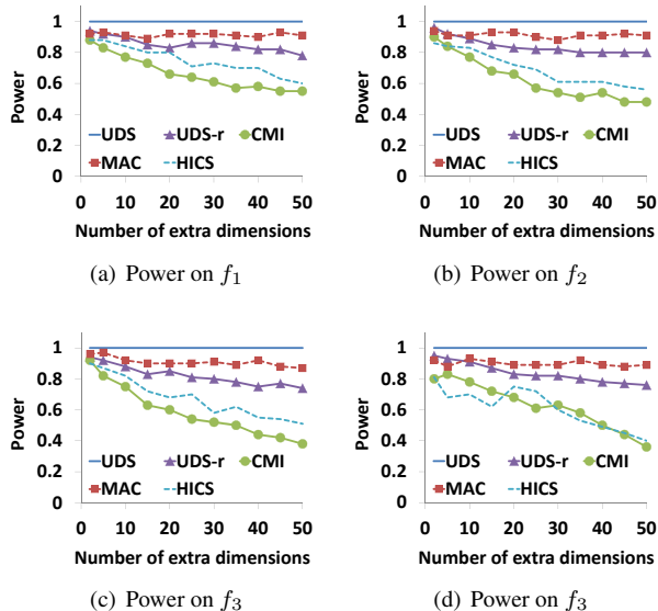
Figure 2: [Higher is better] Statistical power on synthetic data sets for the setting where m = 4000 , n = 20 , and e is varied.
