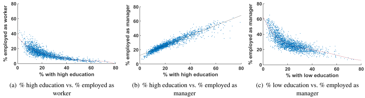
Figure 3: Examples of correlation found by UDS on demographic data. Of the competitors, only MAC can discover these correlation patterns.
