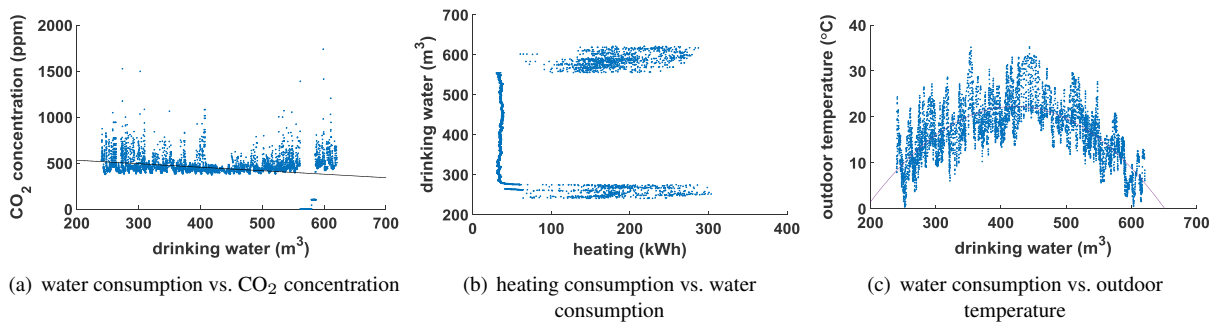
Figure 4: Examples of correlation found by UDS on climate data. Of the competitors, only MAC can discover the first correlation pattern.
