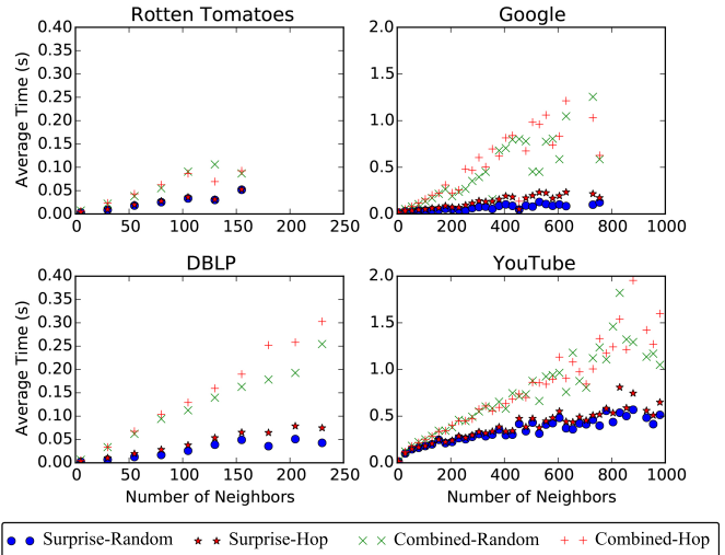
Figure 6: FACETS ranks neighbors in linear time, which is necessary to handle the large numbers of nodes that a user may explore. We show the average time to calculate the JS divergence for surprise and the combination of surprise and interest over a neighborhood of size n . FACETS uses the combined ranking if the user has explored enough to have a user profile from which we can extract the subjective interest ranking. We tested with contiguous node ordering to simulate normal exploration and random ordering to simulate a user searching using the table view.
