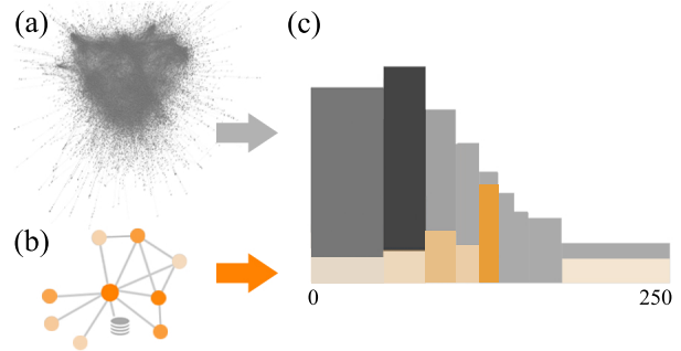
Figure 1: Local and global distribution histograms are both essential to AdaptiveNav. Local histograms (orange bars) are representations of feature distributions (e.g., neighbors’ degree distribution) in a single node’s egonet. The global distributions (gray bars) depicts the corresponding feature’s distribution across the whole graph. The difference between those two distributions reflects if a node is ‘unusual’ or surprising compared to the majority in the graph.
