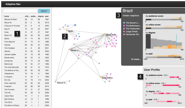
Figure 2: The AdaptiveNav user interface displaying an explored portion of the RottenTomatoes similar-movie graph. The user has traversed several films (shown as orange nodes with titles) and AdaptiveNav has displayed a subset of the relevant neighbors (the nodes with colors ranging from blue to red) and their connectivity. Figures are viewed best in color.
